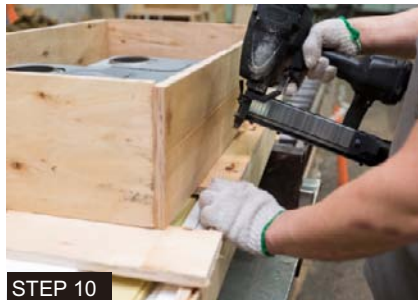
STEP 10 Enclose the sink with slats and attach the 4 slats with the nail gun.
