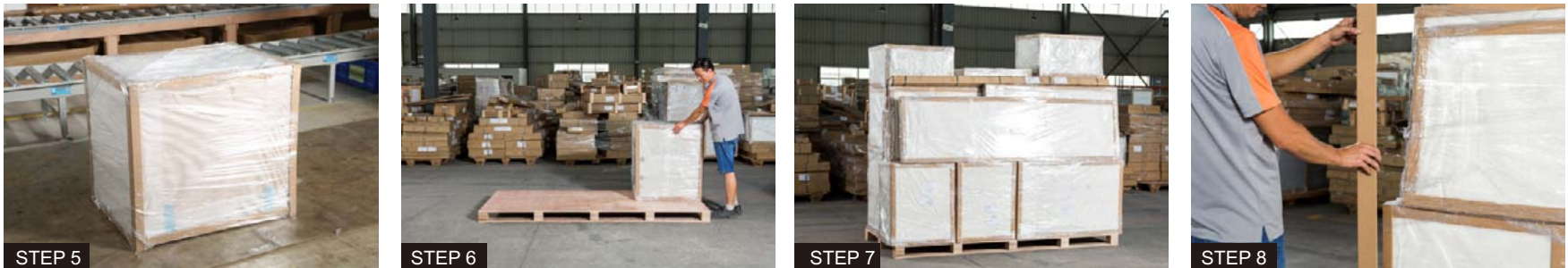
STEP 5 Label the cabinet with shipping mark. STEP 6 Stack pre-assembled units orderly from one side to another side. Packed units must NOT exceed pallet boundary. STEP 7 In order to keep the stacks stable, make sure the stack height is less than 2350mm (including the pallet height). STEP 8 Cover the 4 side edges with cardboard edge strips, then fix it with tape.
