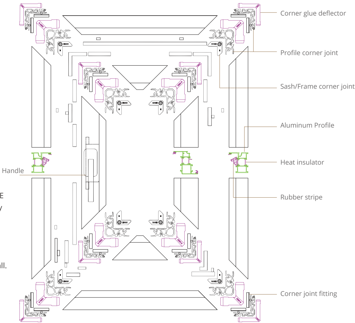
Structure of Tilt and Turn Windows in ZEUS Series
